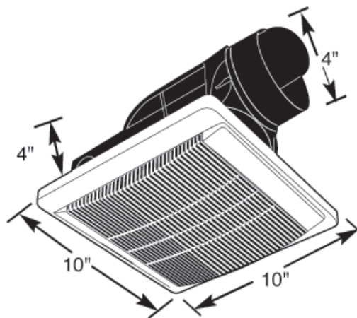
NuVent Product Performance Model NXPF90
