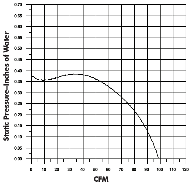
NuVent Product Performance Model NXPF90
